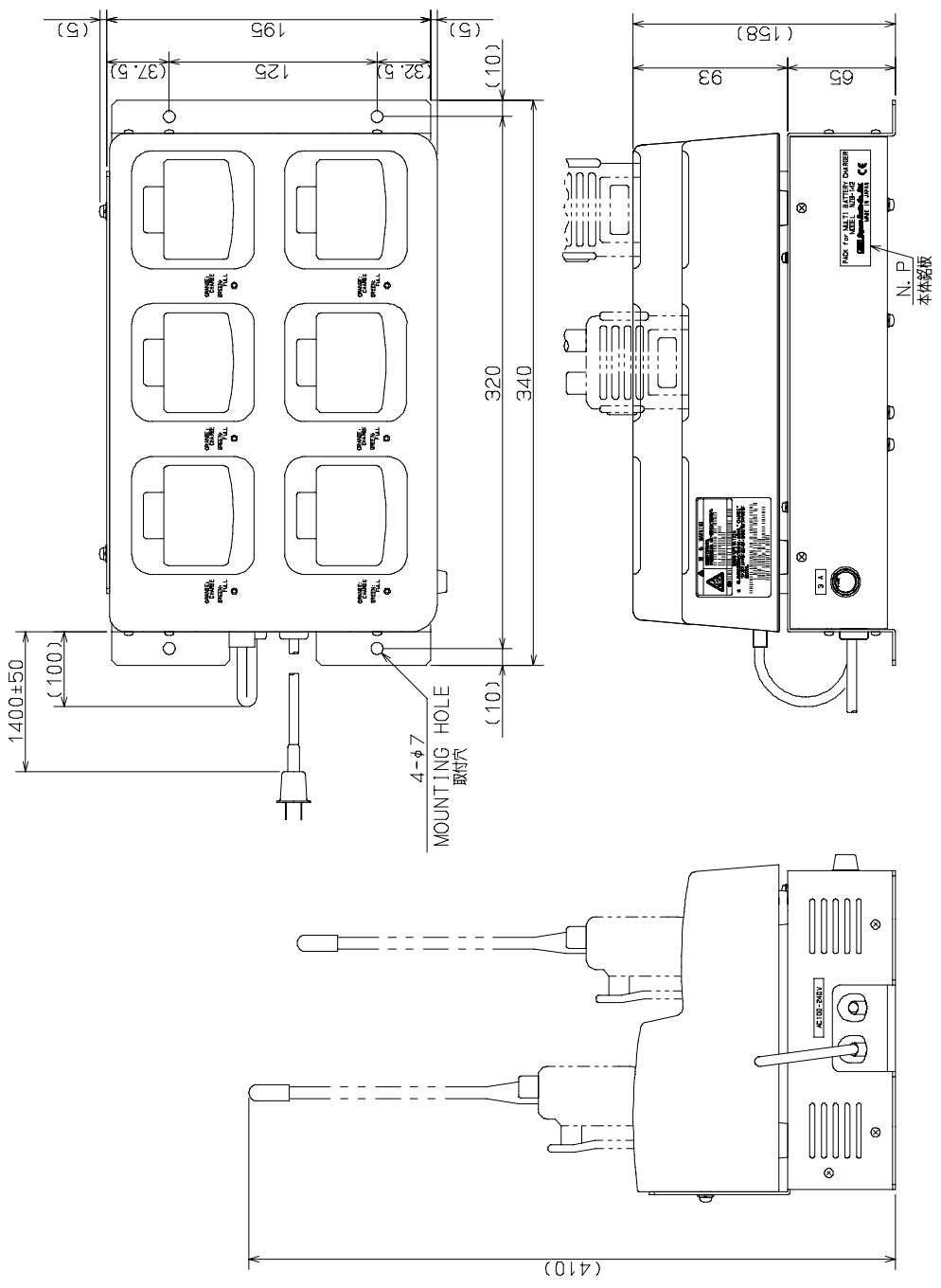
NZB-142 CHARGER FOR 6 BATTERYS (DESKTOP MOUNT TYPE) OUTLINE DRAWING
