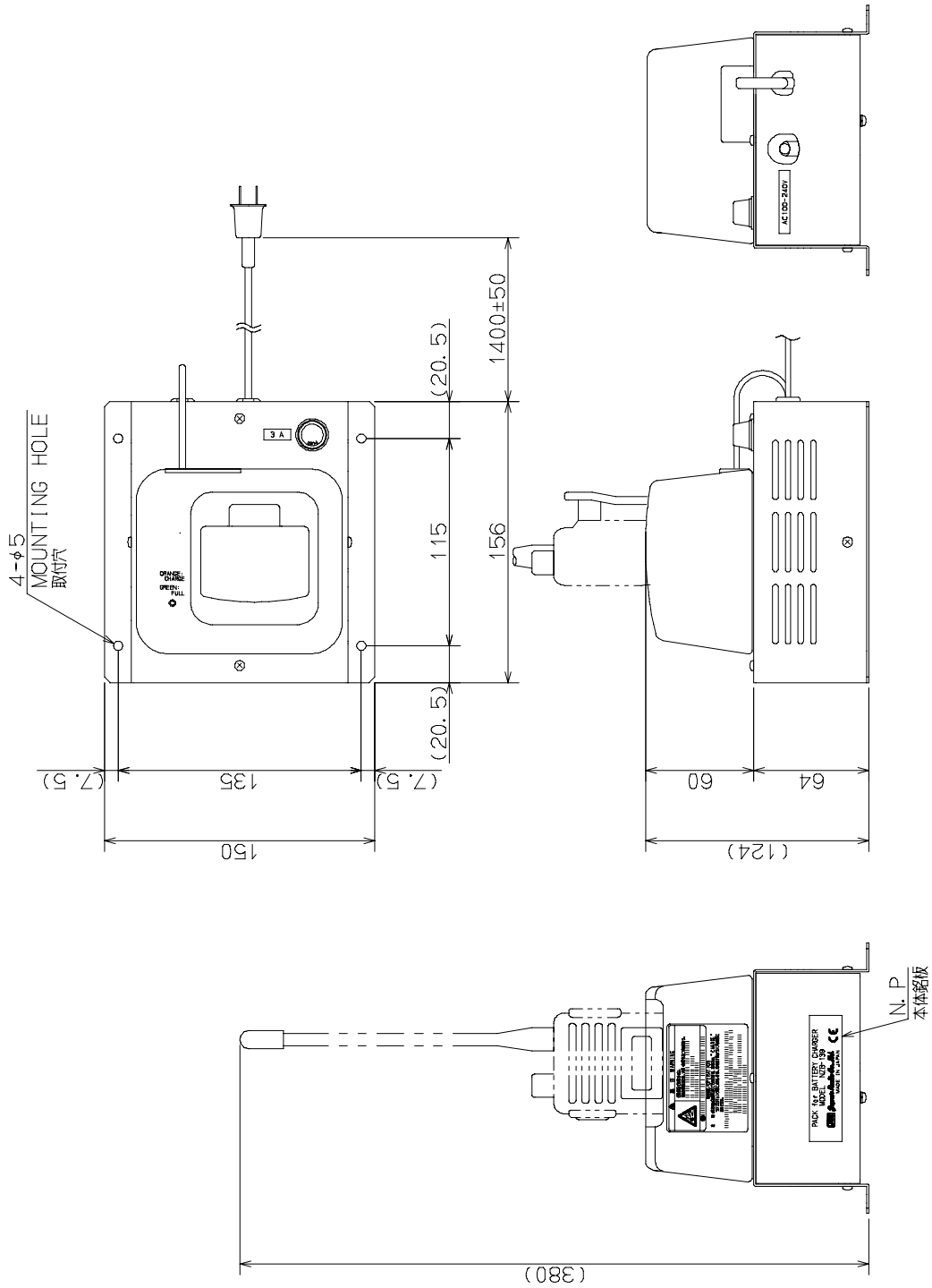
NZB-139 BATTERY CHARGER (DESKTOP MOUNT TYPE) OUTLINE DRAWING
